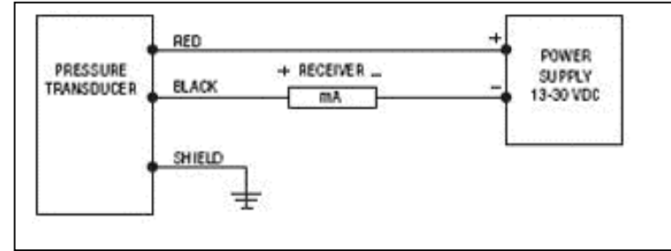
Current Output
